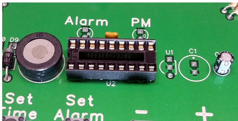
Figure 19 – BZ1 and C2 installed – note their orientation
