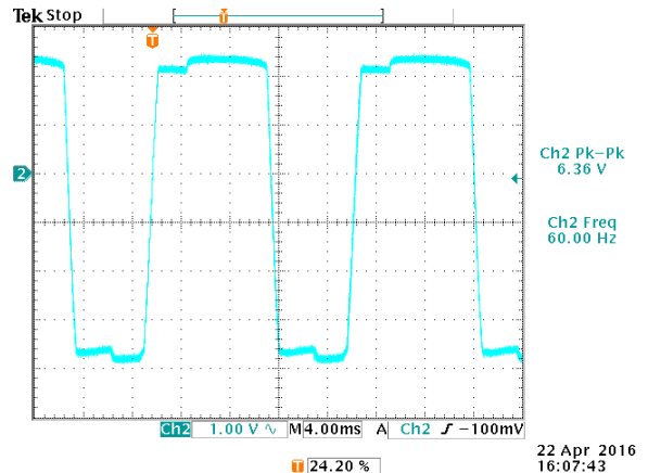
Figure 44 – Clamped 60Hz AC waveform
