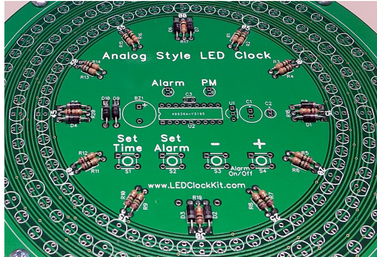
Figure 13 – Installing D1-D10
