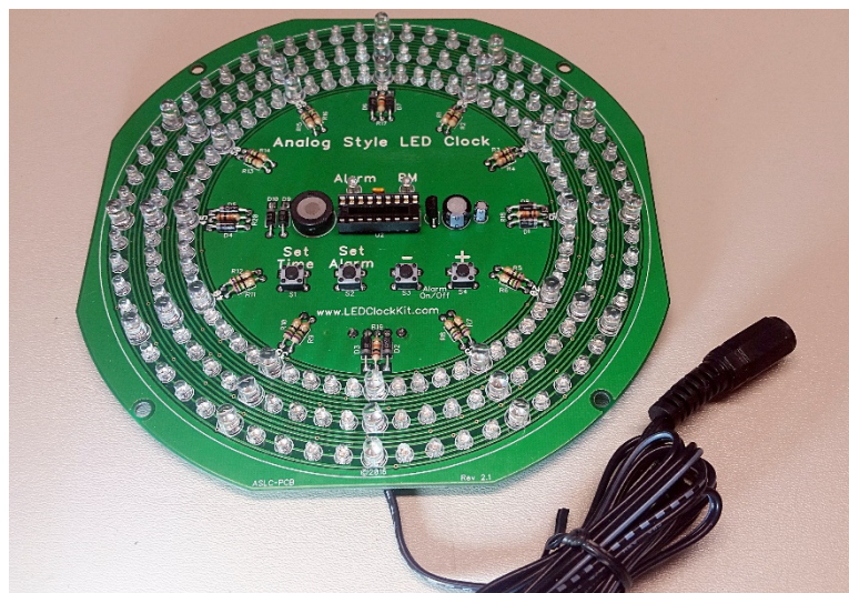
Figure 37 – Completed PCB
