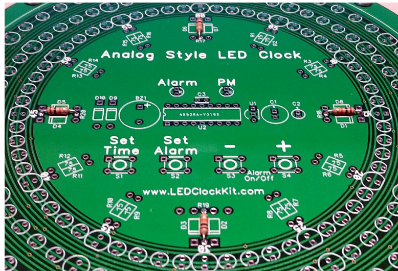
Figure 11 – Installing R17-R20
