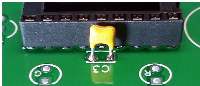
Figure 15 – C3 Installed
