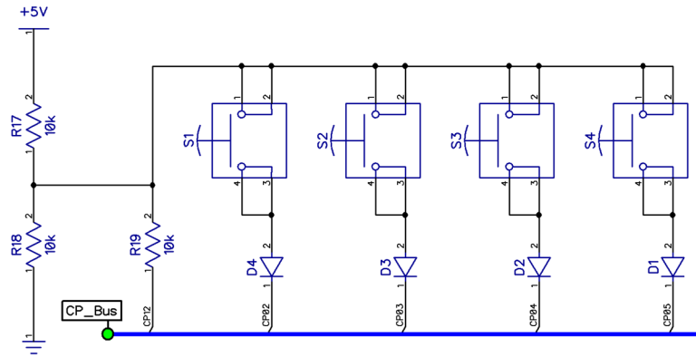
Figure 50 – Schematic, Pushbuttons
