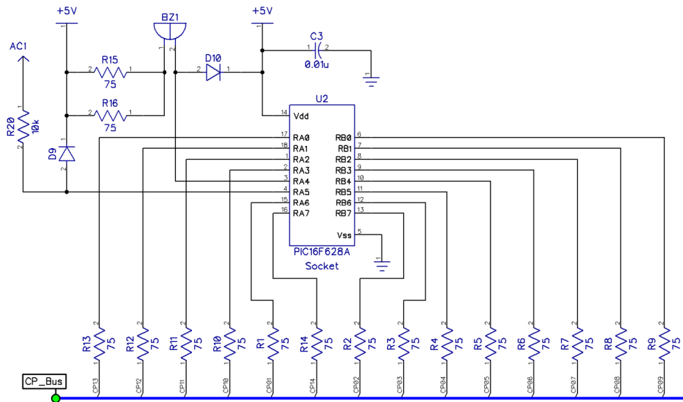
Figure 48 – Schematic, Microcontroller
