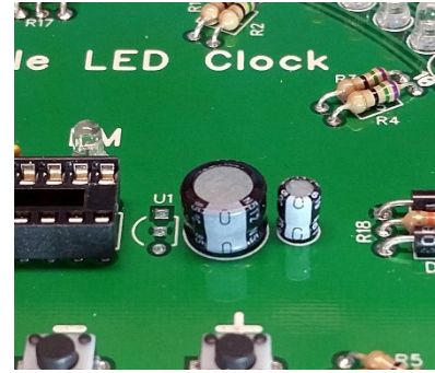
Figure 31 – C1 installed
