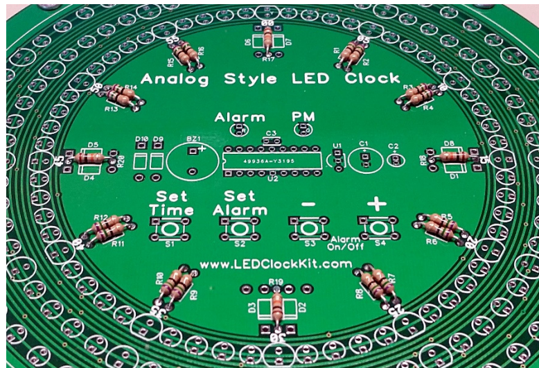
Figure 12 – Installing R1-R16
