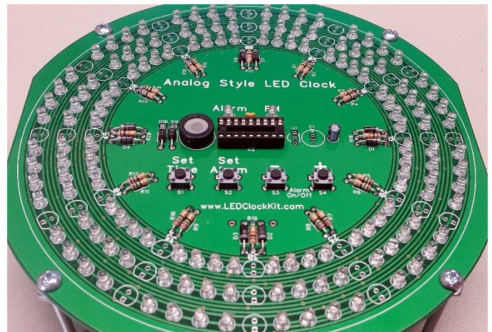
Figure 29 – All 3mm Yellow LEDs installed
