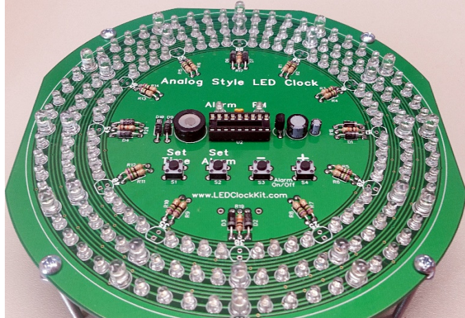
Figure 34 – All 5mm Green LEDs installed
